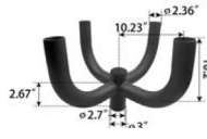
Triple 180° Horizontal Tenon Adapter NO. RB2.5TR180-D
