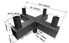
Quad 90° Horizontal Tenon Adapter NO. QT90-4T-D
