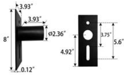
2 3/8 " OD Horizontal Tenon Mid-Pole Bracket NO. ADP2.5-D
