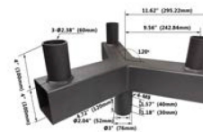
Triple 120° Horizontal Tenon Adapter NO. QT120-3T-D
