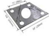
Screw Positioning Plate NO. SPP-D
