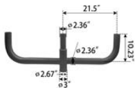
Triple 180° Horizontal Tenon Adapter NO. RB2.5TR180-D
