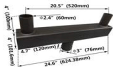
Low Profile Bullhorn with 2 Tenons NO. VTS4R-2T-D
