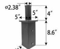
5" Square Pole Mount with 2 3/8 " O.D. Tenon NO. VTS5-D
