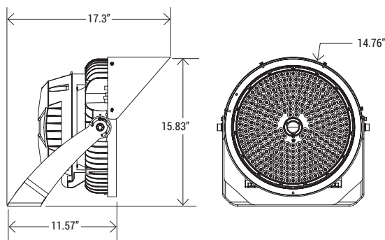
ASA-S (Trunnion)
