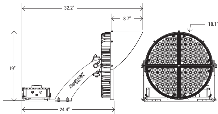
ASA-L (Trunnion)
